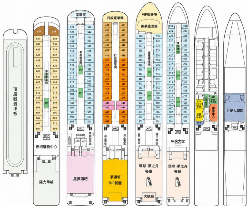
7F頂層甲板 Top Deck 6F陽光甲板 Sun Deck 5F娛樂甲板 Bridge Deck 4F行政甲板 Executive Deck 3F遊步甲板 Promenade Deck 2F上甲板 Upper Deck 1F主甲板 Main Deck -1F艙底 Lower Deck
